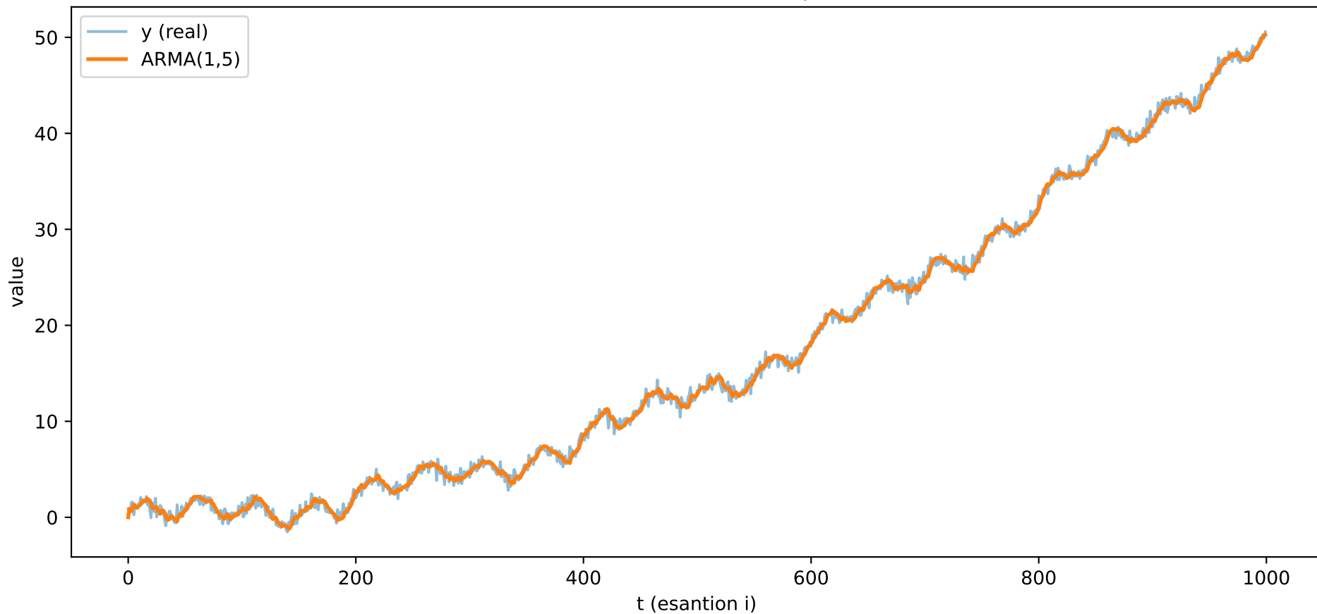
Predictii model ARMA optim
